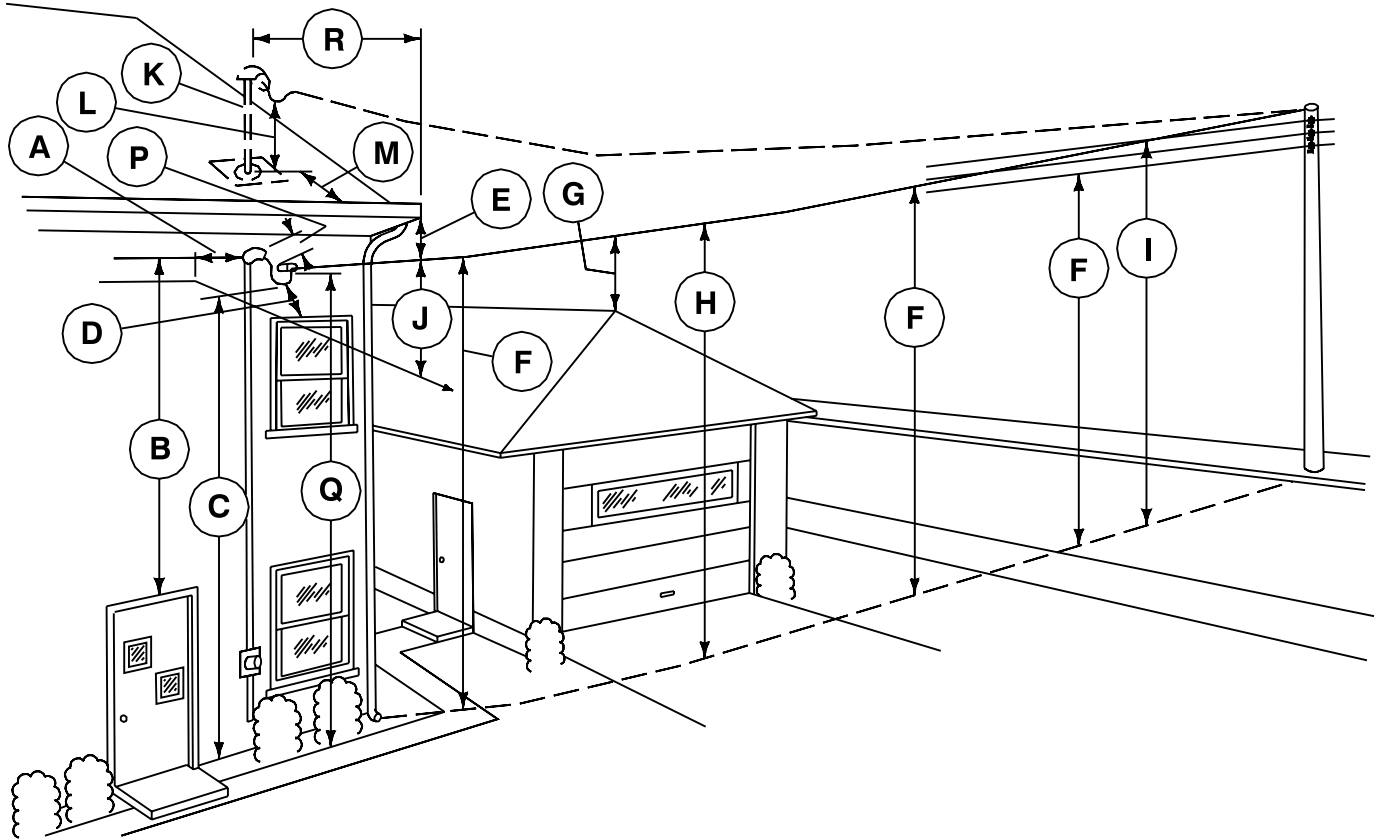
MINIMUM CLEARANCE
